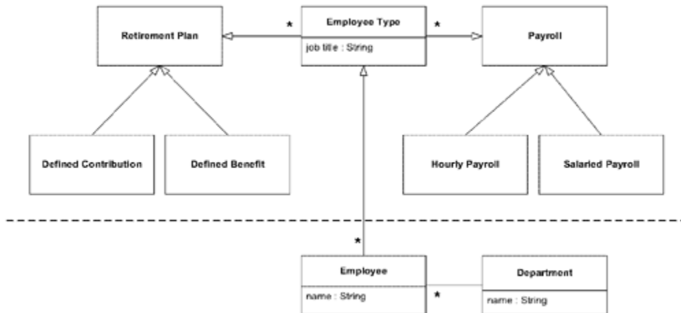
Figure 16.22. Payroll is now explicit, distinct from Employee Type.
